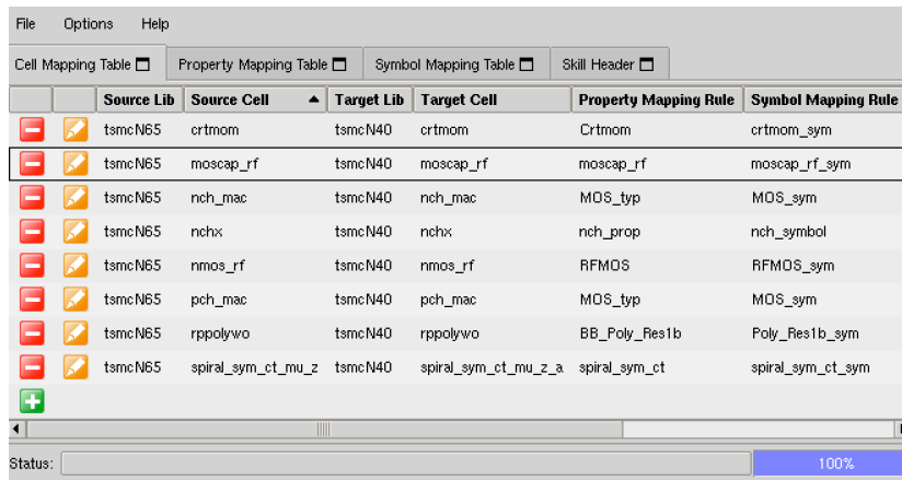
Schematic Porting Tool GUI 화면 예시 (TSMC 65nm -> TSMC 40nm)
