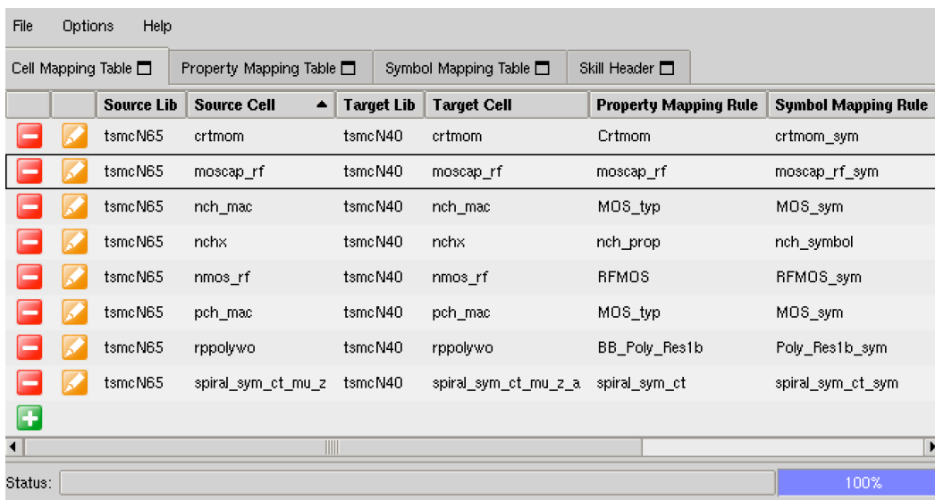
Schematic Porting Tool GUI 화면 예시 (TSMC 65nm -> TSMC 40nm)
